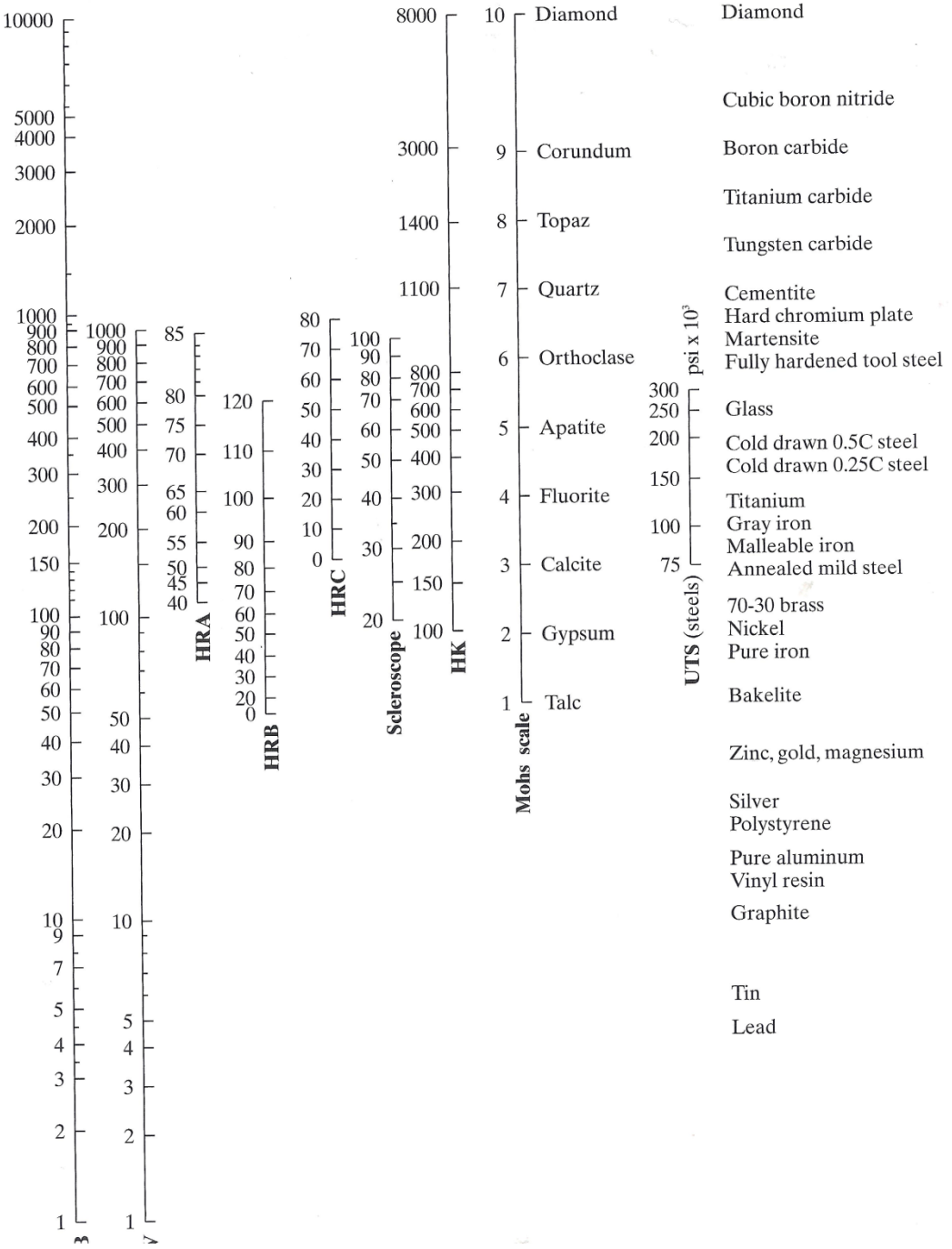
FIGURE 2.14 Chart for converting various hardness scales. Note the limited range of most scales. Because of the many factors involved, these conversions are approximate.
